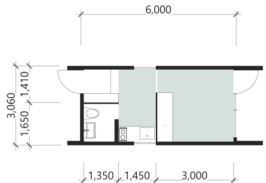
FLOOR PLAN
